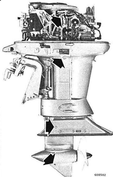
Figure 2-15. Port Side
